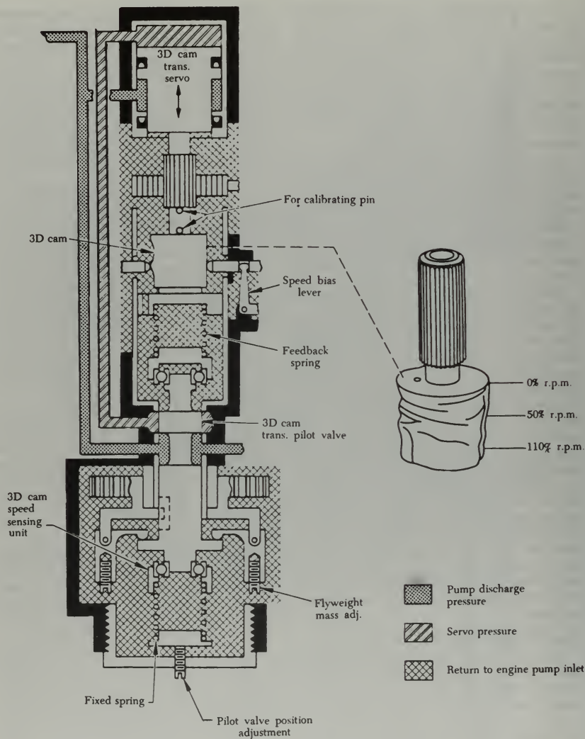
FIGURE 3-52. Three-dimensional cam and translating unit.
